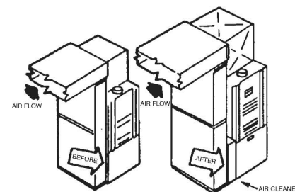
OFFSET INSTALLATION If there is less than 7-in. for mounting the air cleaner between the duct and the furnace, move the return air drop.
